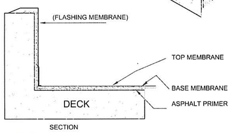
DETALLE #1
